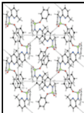
Fig. 2. Depiction of C—H...O interactions in the title compound(I)
